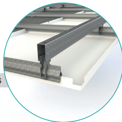
Detail of hanging panels
